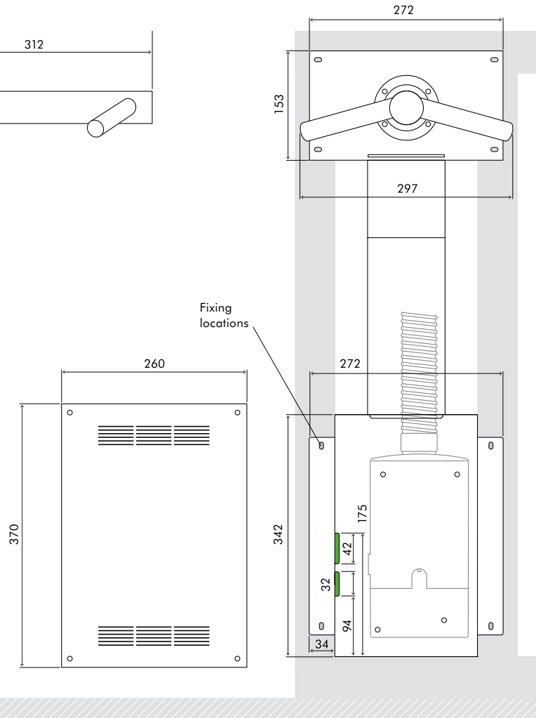
REAR ELEVATION
