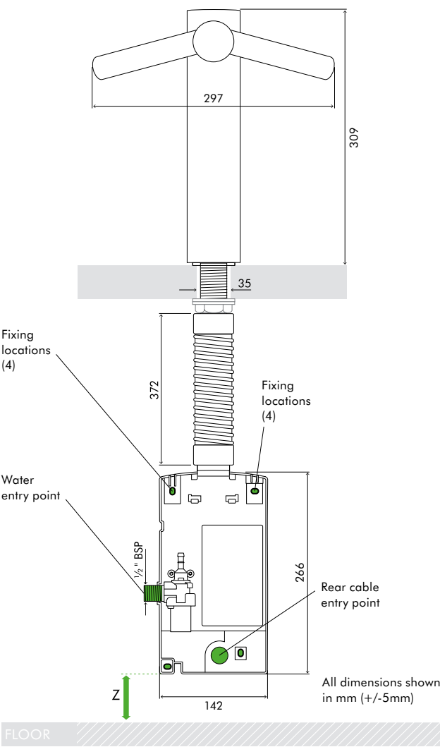
REAR ELEVATION
